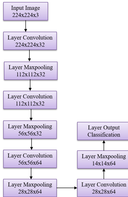
Figure 5. Third CNN Architectural Model
