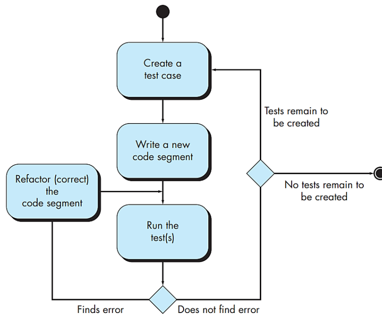
Figure 1. Test-driven development (TDD) method
